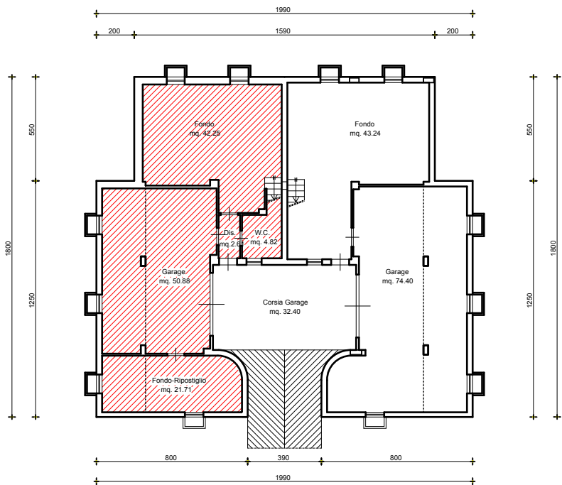
PIANO SEMINTERRATO
