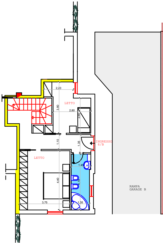
PIANO TERRA
